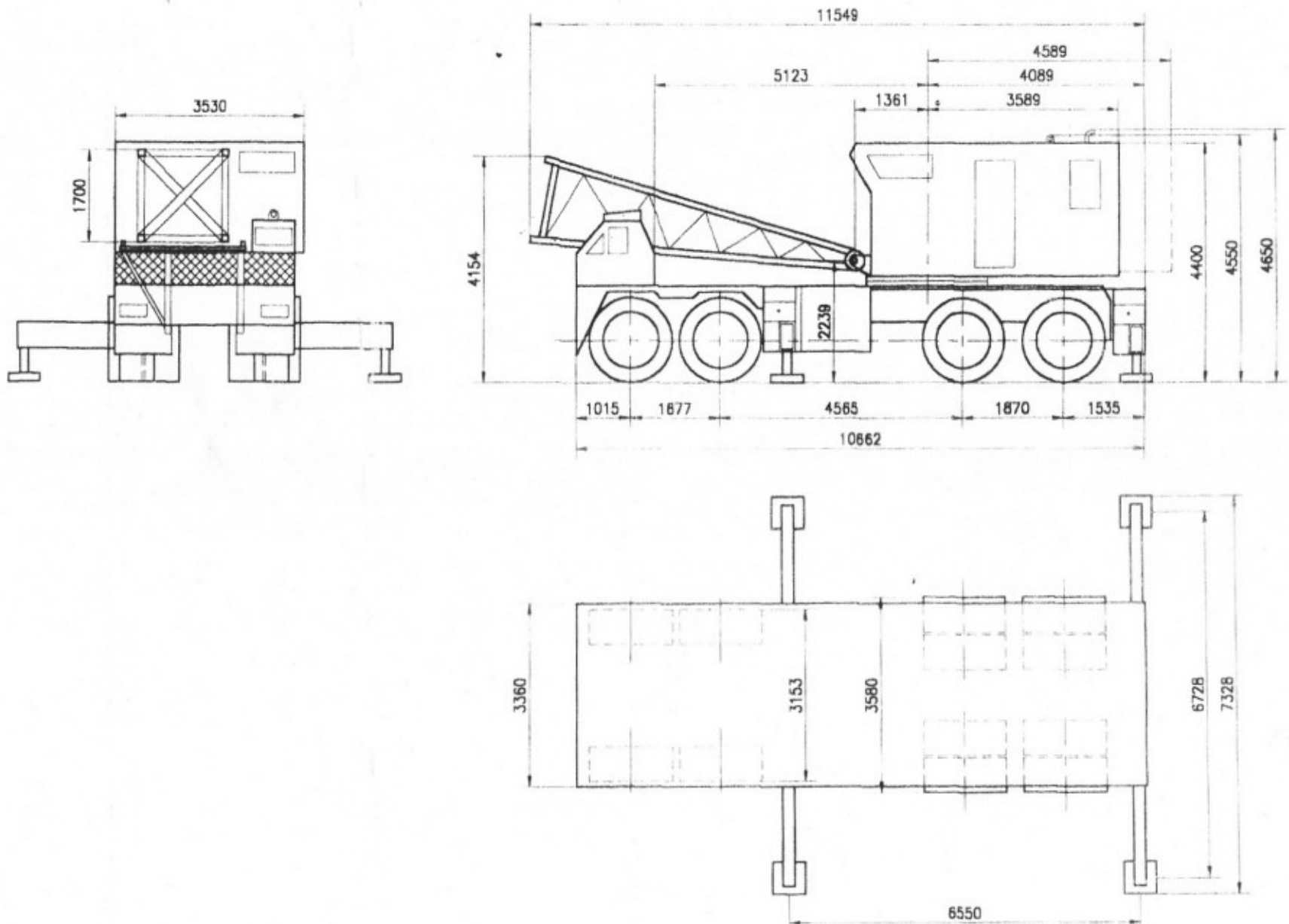
NATIONAL OS-435. TRUCK MOUNTED LATTICE BOOM CRANE
